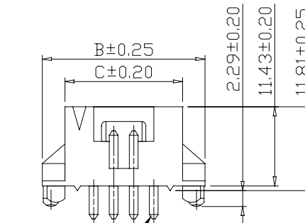
PIN0.64SQ, Circuit 1
